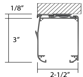
Ceiling mount bracket
