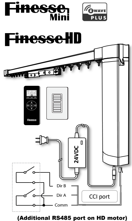
(Additional RS485 port on HD motor)
